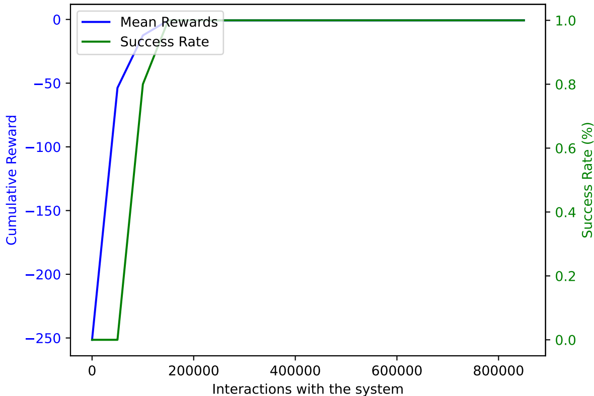
TRPO on AWAKE with DoF: 5 and trained on 850000 samples averaged over 10 validation episodes
