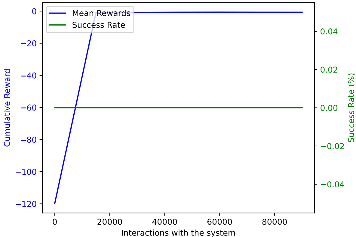
TRPO on AWAKE with DoF: 5 and trained on 90000 samples averaged over 10 validation episodes
