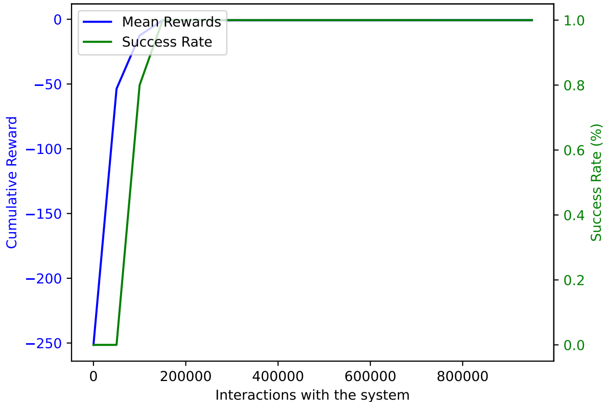
TRPO on AWAKE with DoF: 5 and trained on 950000 samples averaged over 10 validation episodes
