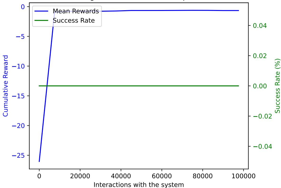
TRPO on AWAKE with DoF: 5 and trained on 97500 samples averaged over 10 validation episodes
