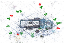
CrossScore
