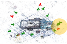
FisherRF
