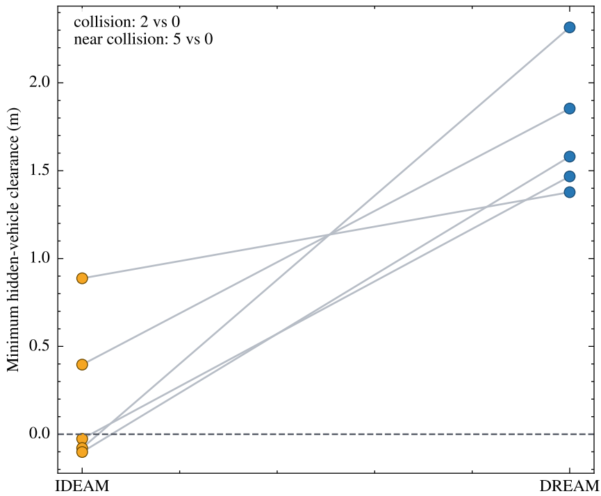
B Paired true-threat safety margin
