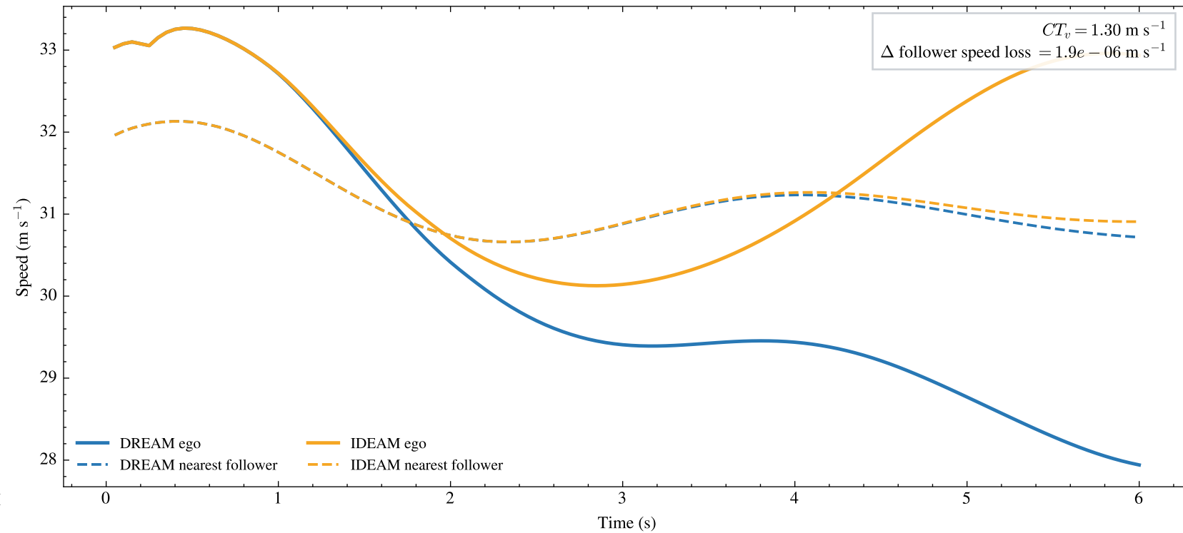
C Empty-shadow ego and trailing-vehicle response
