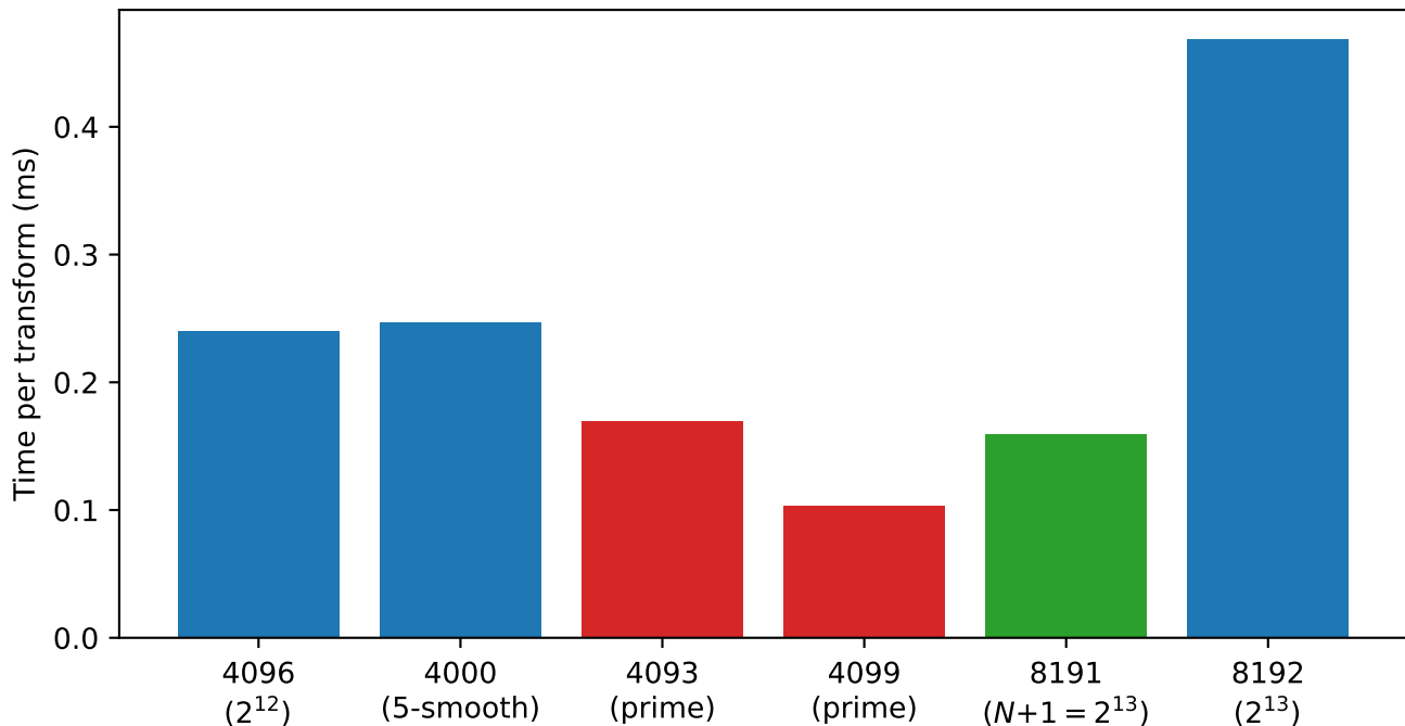
Hankel transform timing vs. grid size (green: N+1 is a clean power of 2; red: N+1 has a large prime factor)
