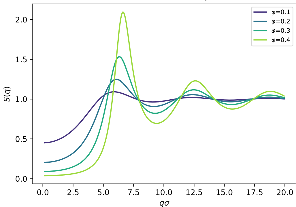
Structure factor S(q)
