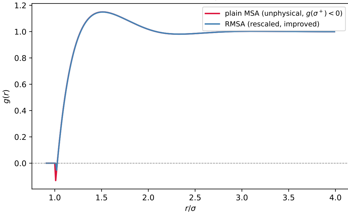
Charged system: MSA breakdown vs. grow-then-bisect RMSA ( \kappa\sigma=3.5 , Z=5.0 , \phi=0.1 )
