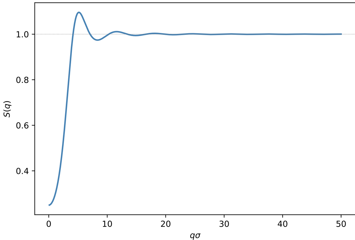
Hayter-Penfold RMSA: charged colloid, \phi=0.1
