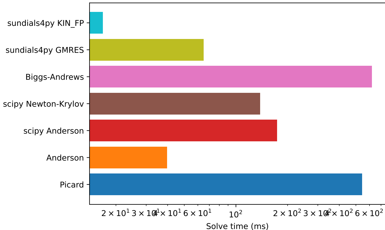
Solver speed comparison, HardSphere+PY, \phi=0.4
