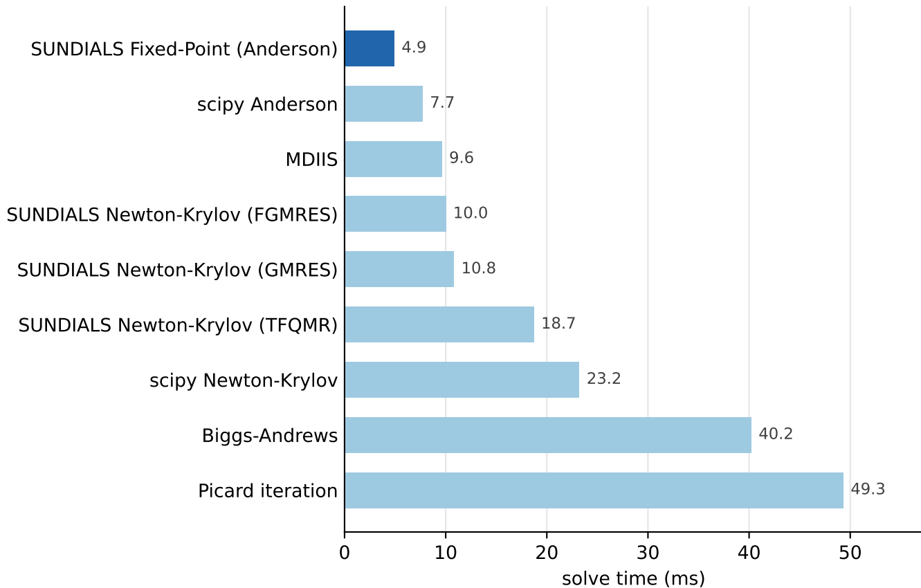
Solver speed, hard spheres, Percus-Yevick
