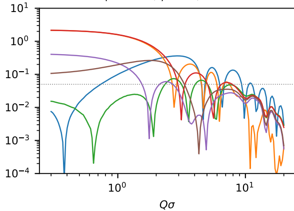
square well, \phi=0.20 , s=0.30
