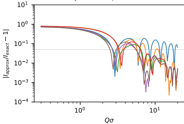
sticky HS \tau=0.3 , \phi=0.20 , s=0.20
