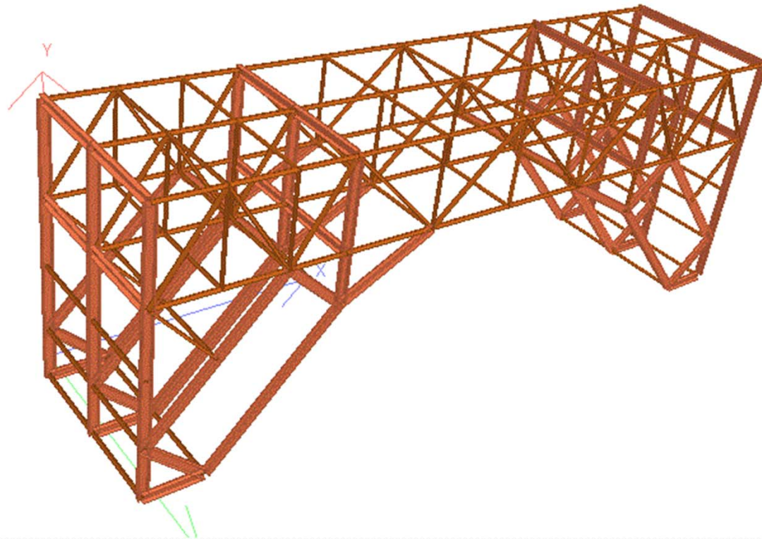
C- Seam RT Shield structure
