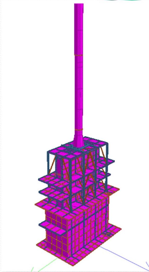
Ketene Furnace
