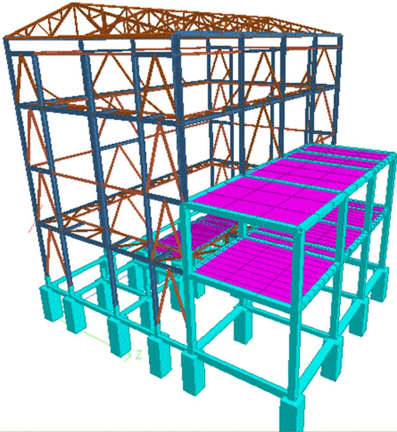
Boiler Plant Structure (Bagasse Fired)
