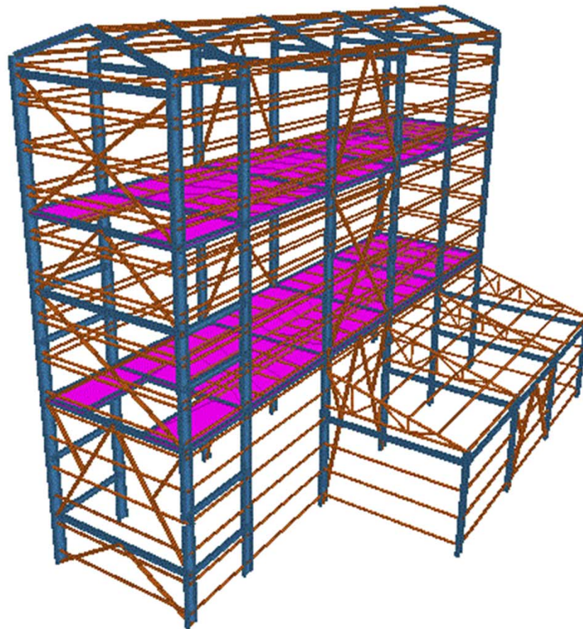
Evaporation Plant Structure
