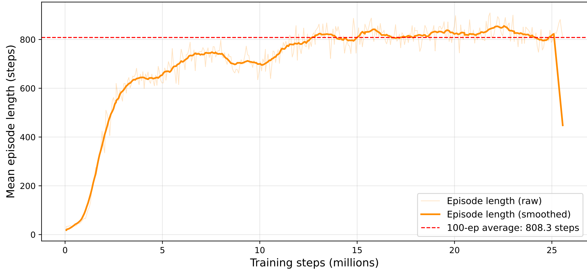
PPO Phase 3 — Episode Length (run 3kupgeme)
