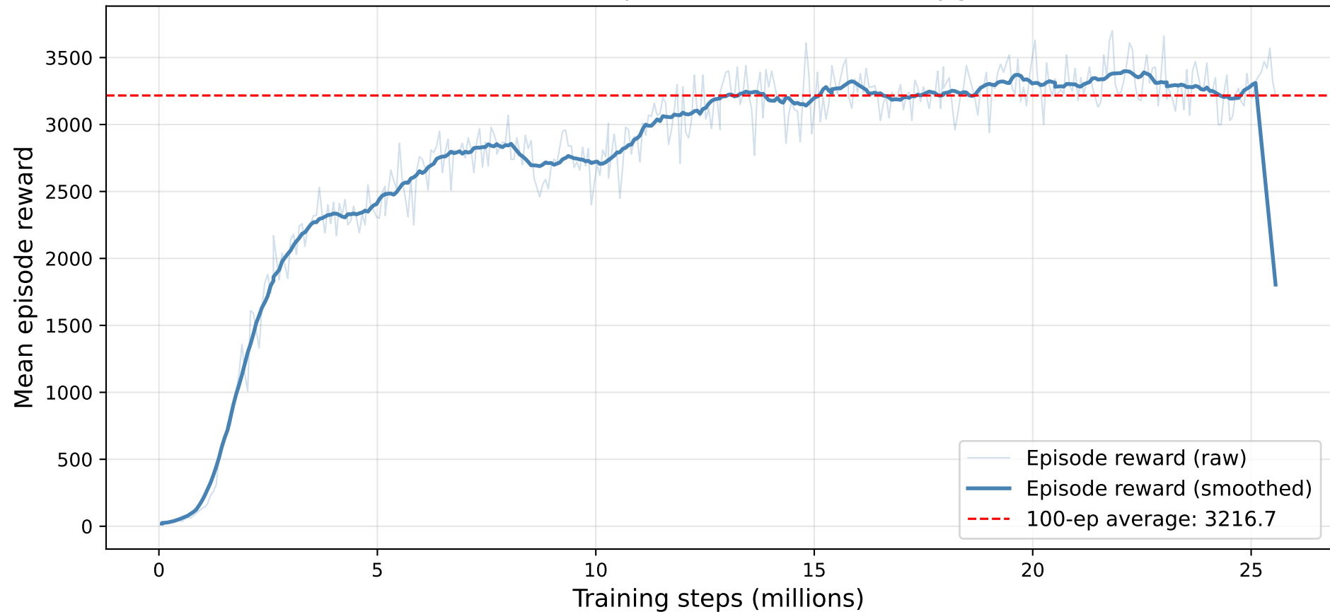
PPO Phase 3 — Episode Reward (run 3kupgame)
