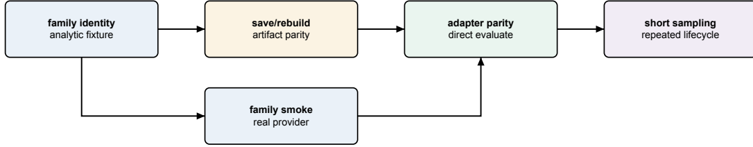
FIG. 11. A common evidence dependency. Identity establishes local mathematics, smoke establishes the real provider path, save/rebuild establishes persistence and adapter/sampling gates establish external use.
