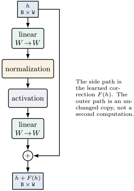
FIG. 5. A residual block. Both paths have the same shape, so addition is coordinate by coordinate. The skip path gives the gradient a direct route around the learned correction.
