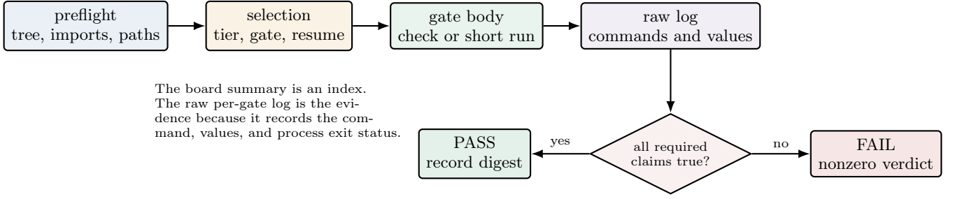
FIG. 10. The board’s evidence flow. Preflight and selection determine what is eligible to run; the gate body produces evidence; the board converts all required claims into one explicit verdict.
