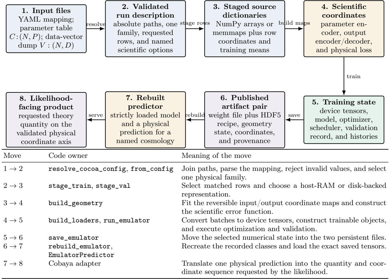
FIG. 1. The complete ownership chain. Blue boxes contain file- or host-side data, gold boxes own reversible scientific coordinates, green owns optimization state, and purple marks a published interface. An arrow names the code that must validate the object crossing that boundary.
