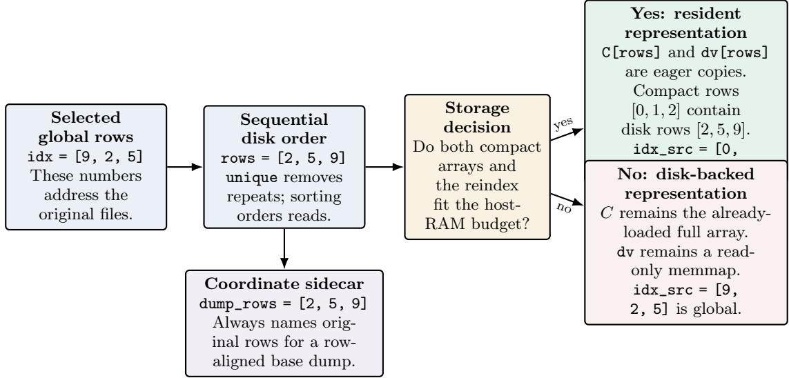
FIG. 4. One selection, two storage representations, and two coordinate systems. A global row addresses the original files; a local row addresses a compact copy. idx_src must be interpreted with the returned C/dv pair. dump_rows never becomes local because the grid2d base file is addressed in original-file coordinates.
