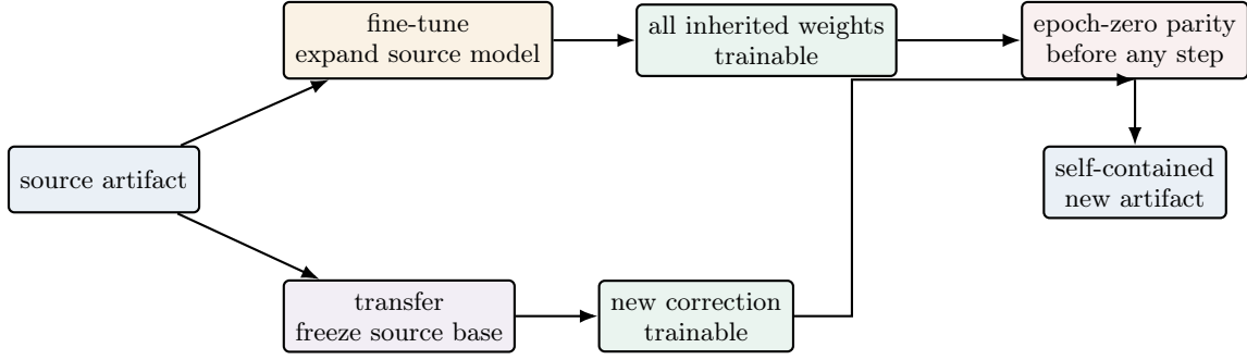
FIG. 9. The two warm-start strategies. They differ in which parameters may move, but both must reproduce the source function before training and publish a self-contained result afterward.
