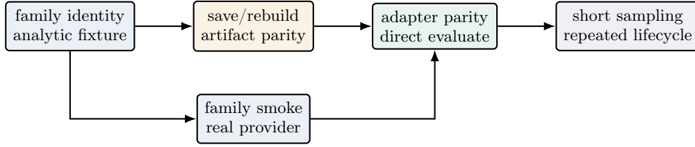
FIG. 11. A common evidence dependency. Identity establishes local mathematics, smoke establishes the real provider path, save/rebuild establishes persistence, and adapter/sampling gates establish external use.
