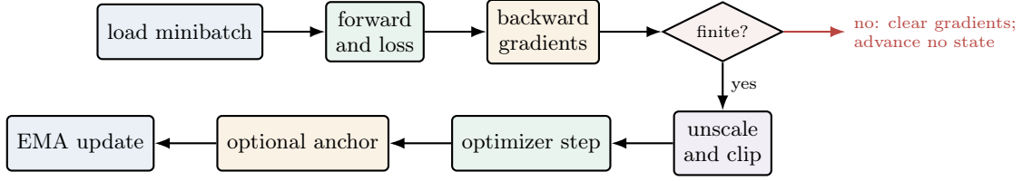
FIG. 8. One accepted training step. The order is part of the algorithm. Finiteness is checked before any persistent state advances; EMA is last because it summarizes the accepted post-step parameters.
