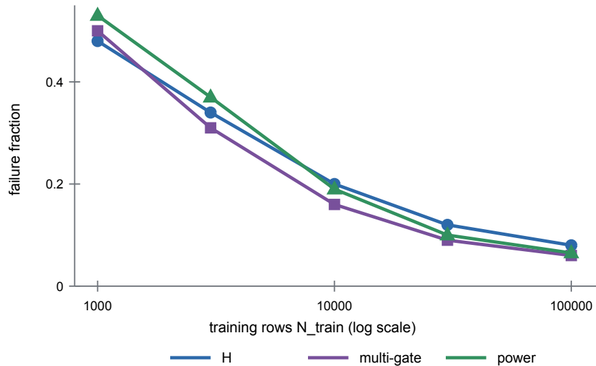
Training-size learning curve
