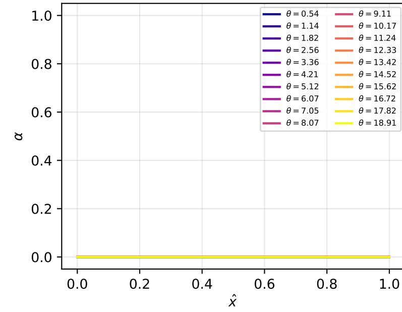
Dynamic: fragmentation generations
