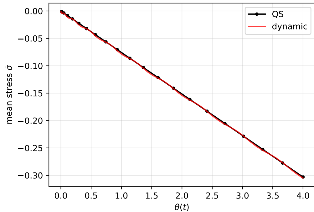
Mean stress vs thermal strain
