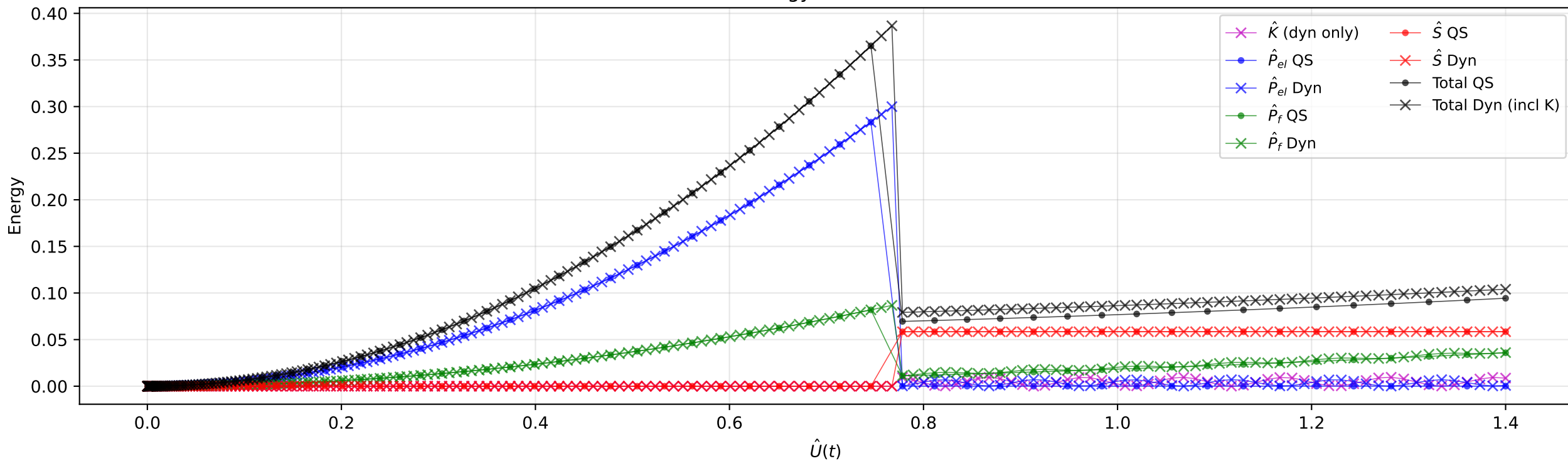
Energy evolution
