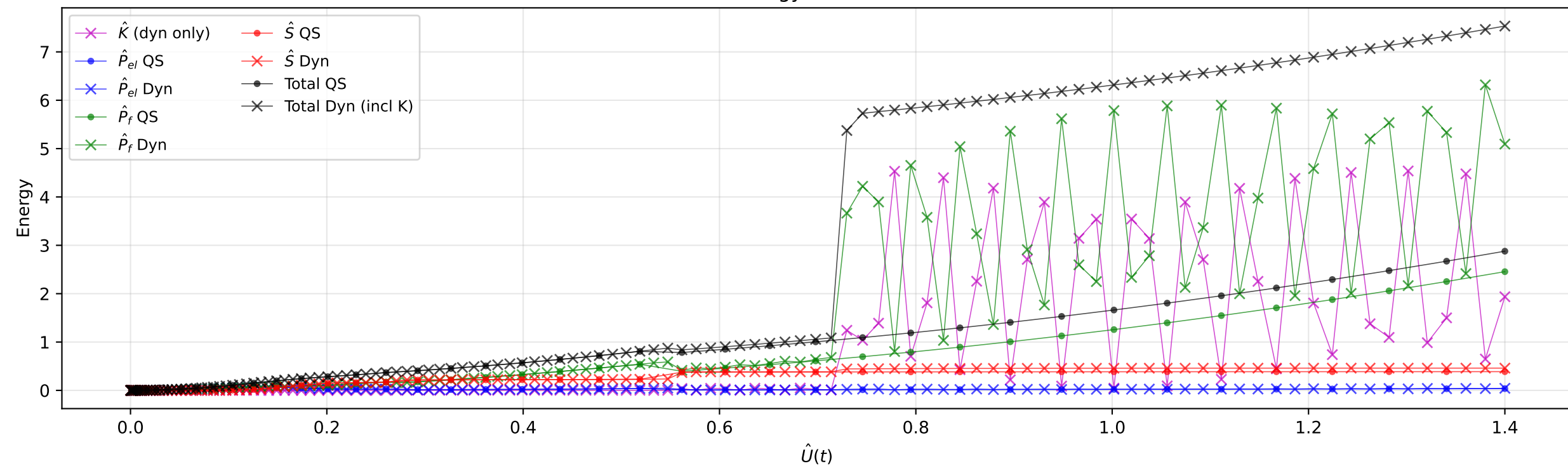
Energy evolution
