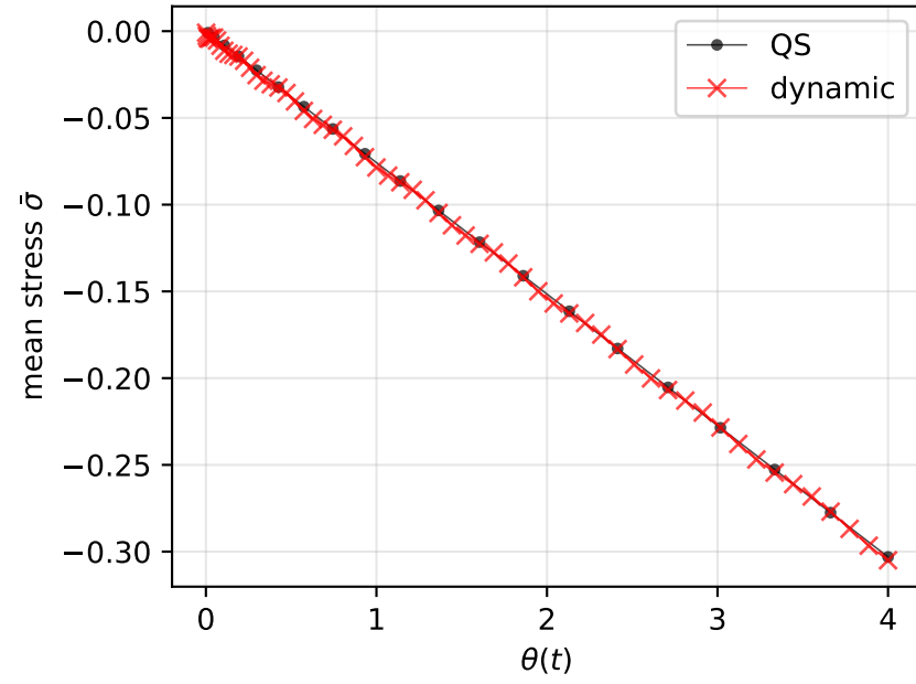
Mean stress vs thermal strain
