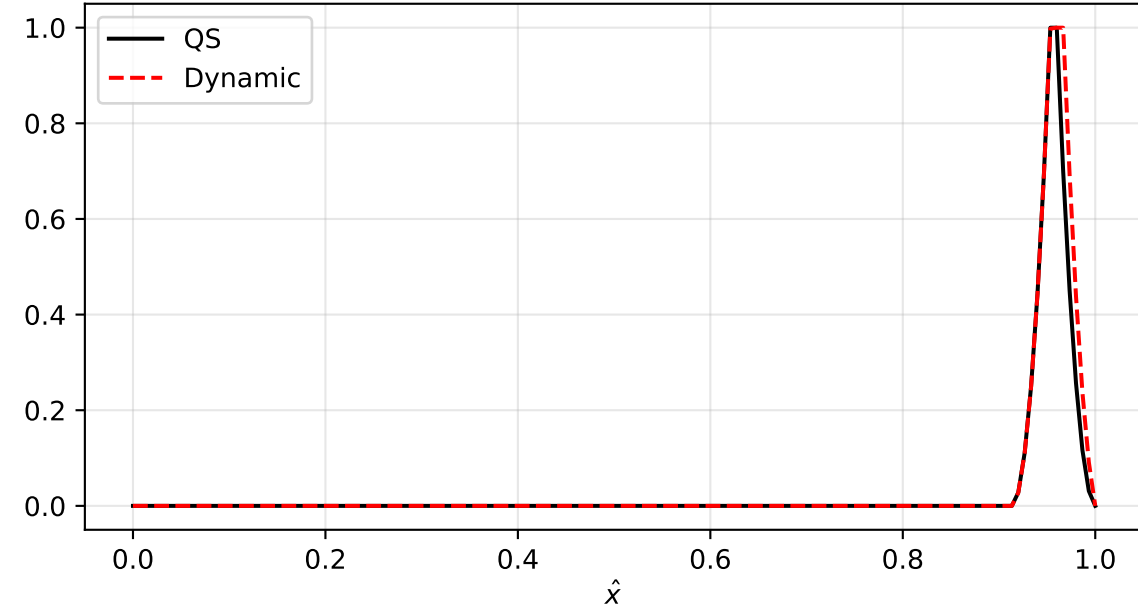
Final damage at \hat{U} = \hat{U}_{\max}
