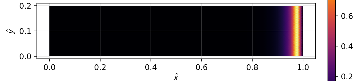
Final damage at \hat{U} = \hat{U}_{\max}
