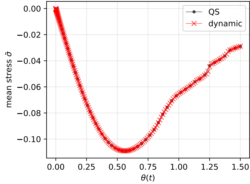
Mean stress vs thermal strain
