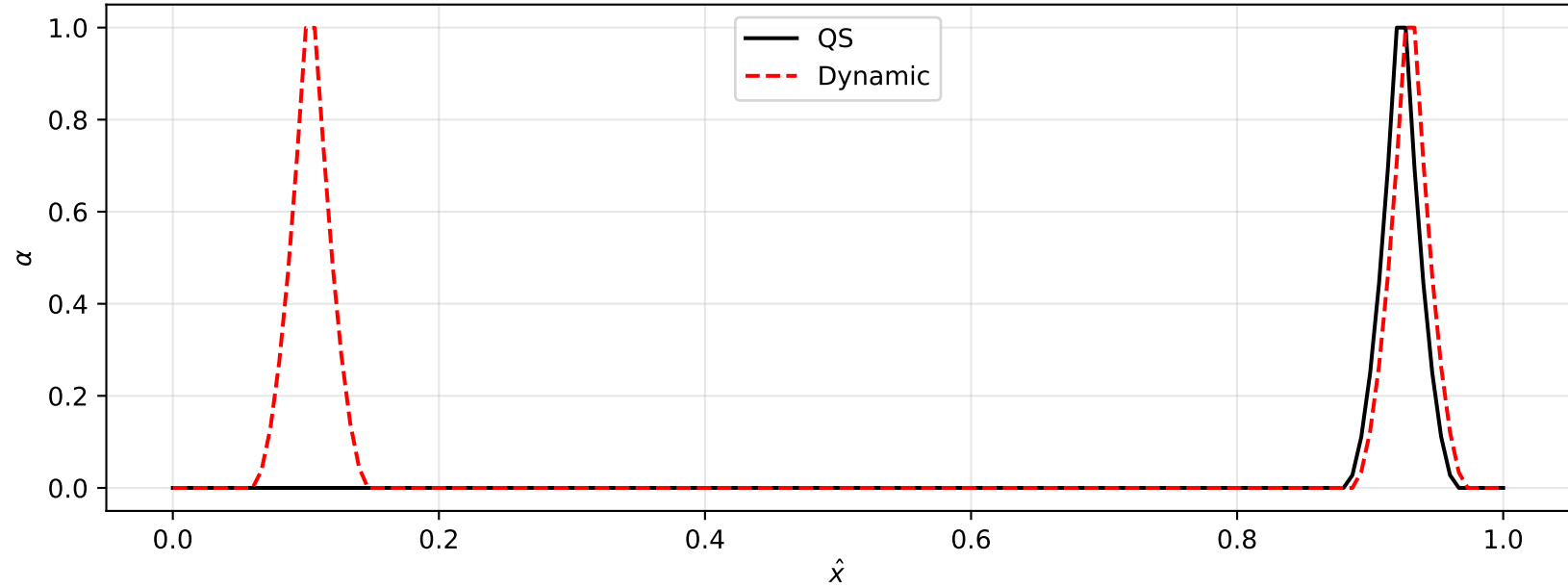
Final damage profile at \hat{U} = \hat{U}_{max}
