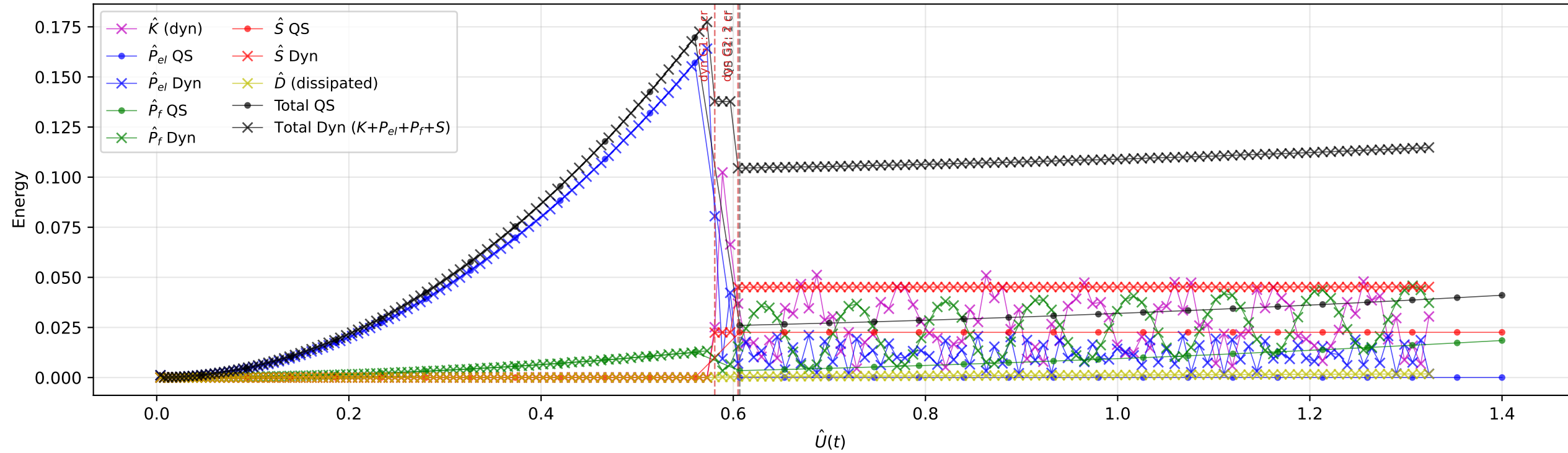
Energy evolution
