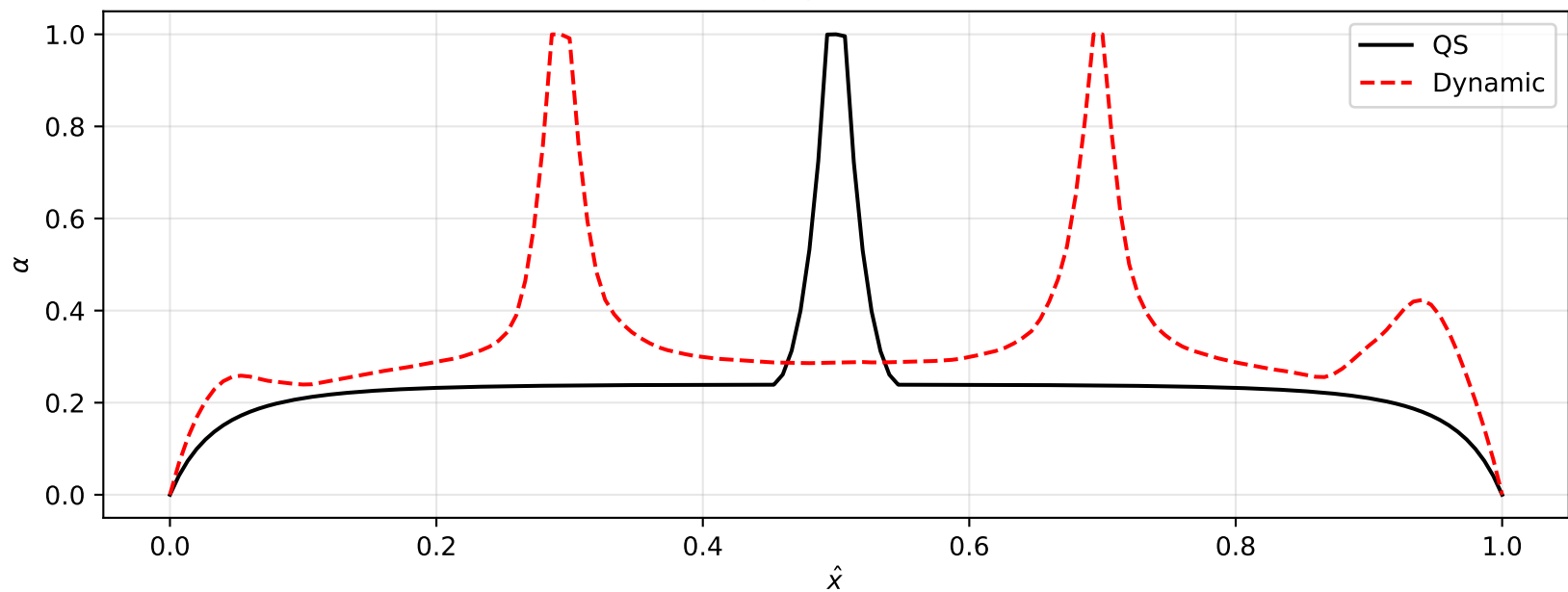
Final damage profile at \hat{U} = \hat{U}_{max}
