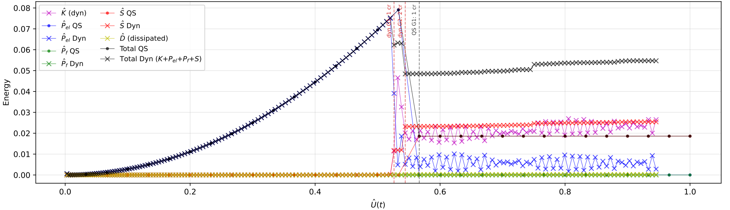
Energy evolution
