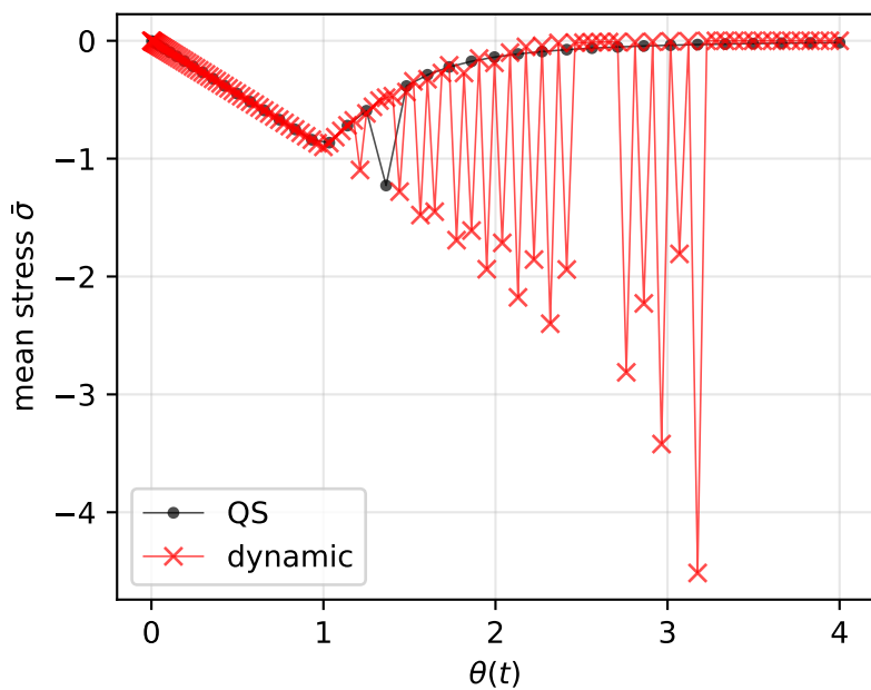
Mean stress vs thermal strain
