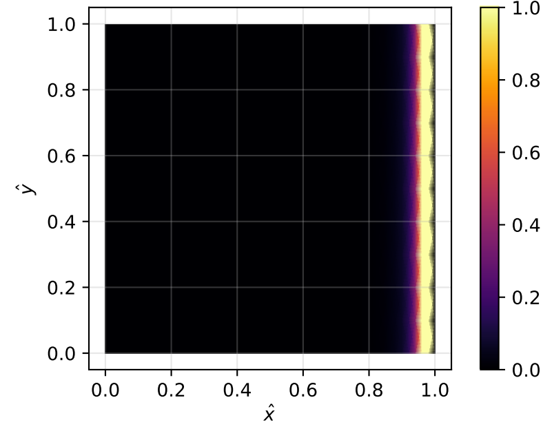
Final damage at \hat{U} = \hat{U}_{\max}
