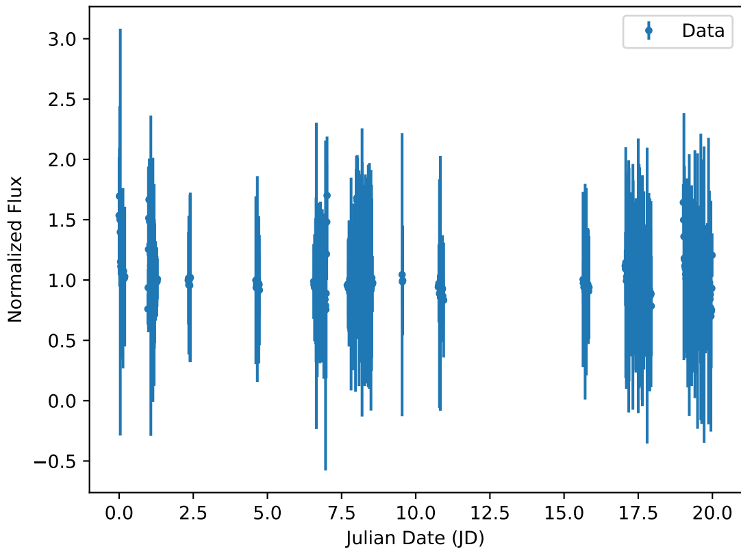
Observed Data
