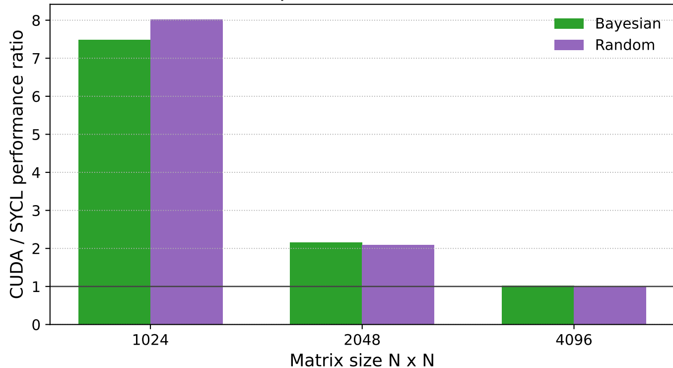
CUDA/SYCL performance ratio - Matmul
