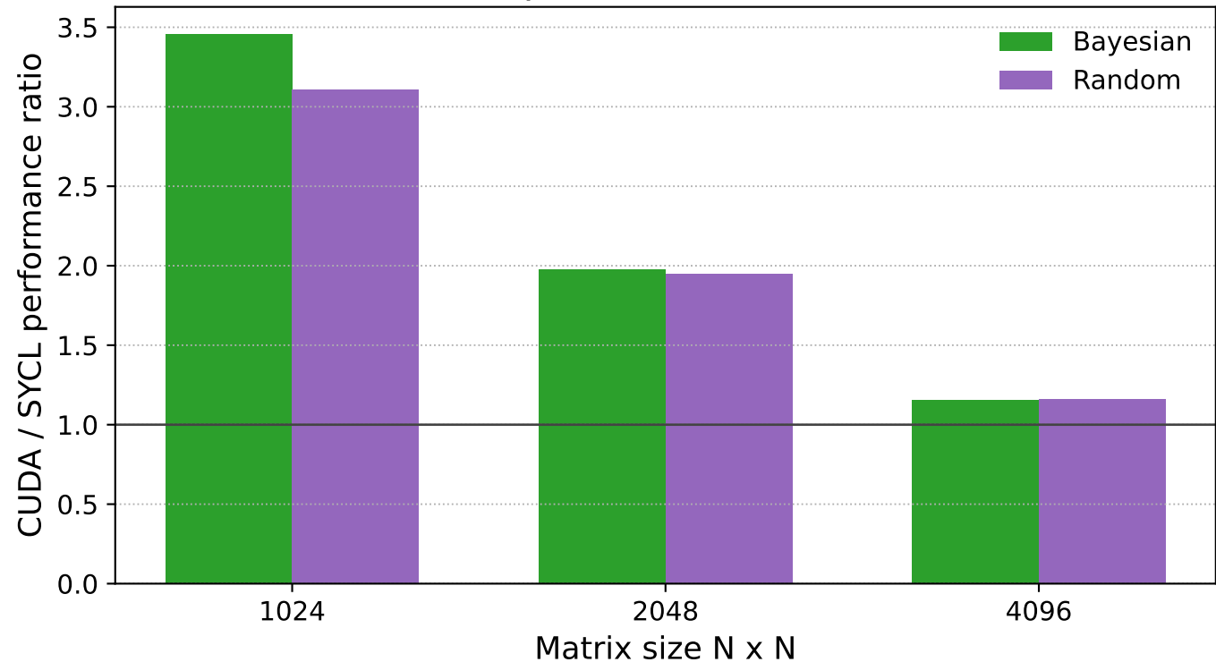
CUDA/SYCL performance ratio - Stencil
