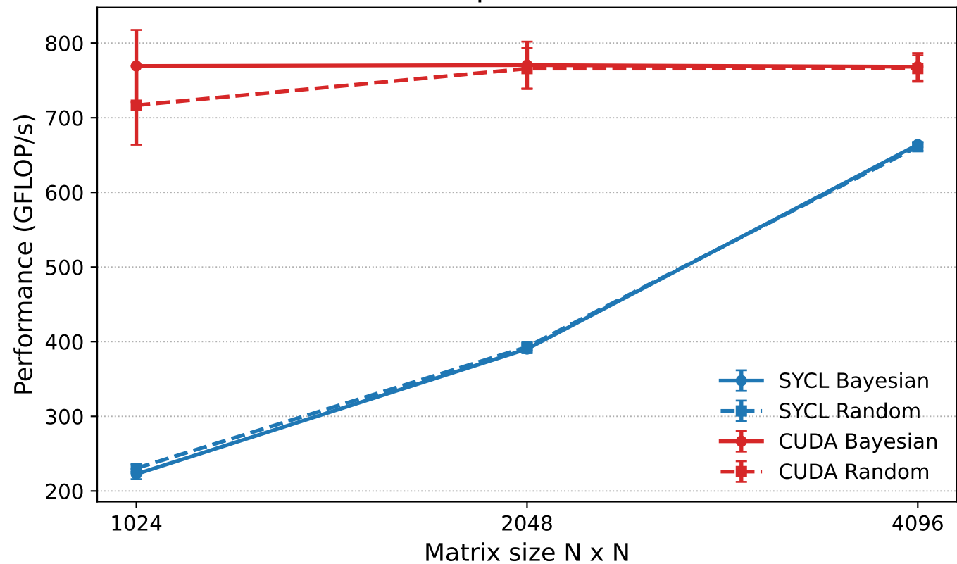
SYCL vs CUDA performance - Stencil
