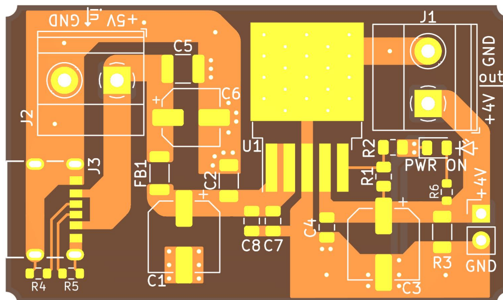
Figure B-1 – PCB Top Copper
