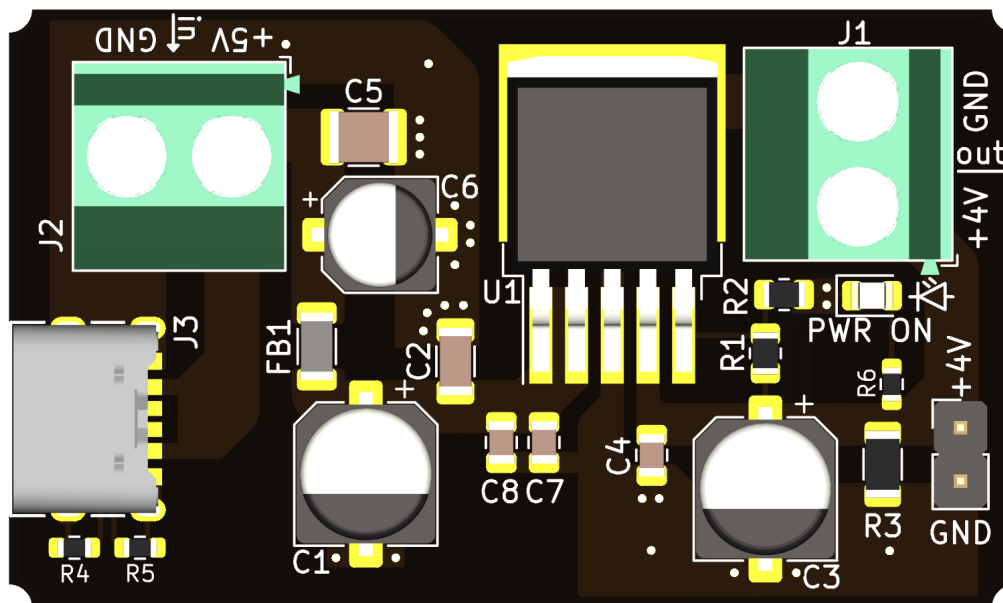
Figure B-5 - 3D Top View
