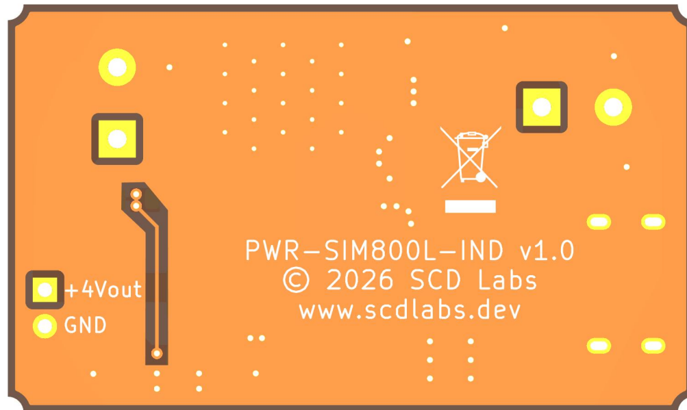
Figure B-2 - PCB Bottom Copper
