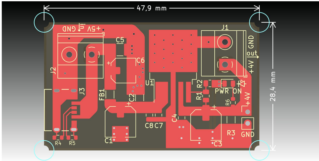
Figure C-1 – Overall PCB Dimensions
