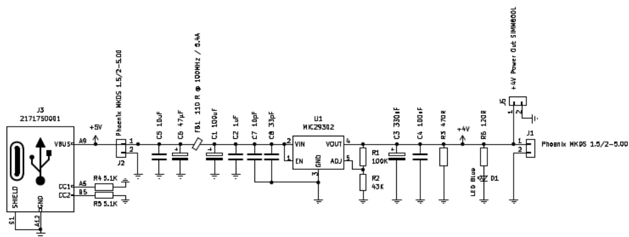
Figure A-1 - Complete Electrical Schematic
