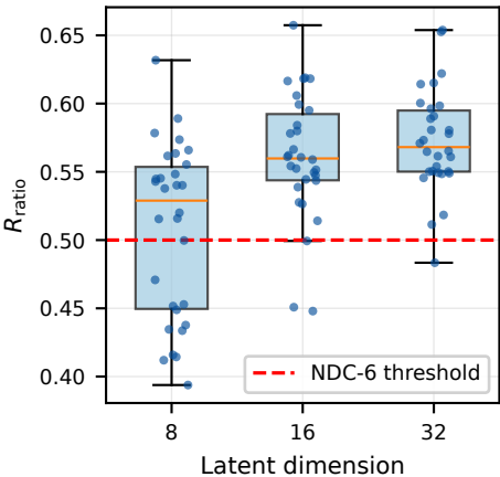
(a) Per-seed R_{\text{ratio}}
