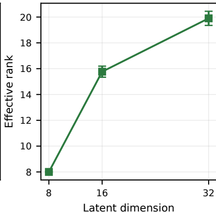
(b) Effective rank
