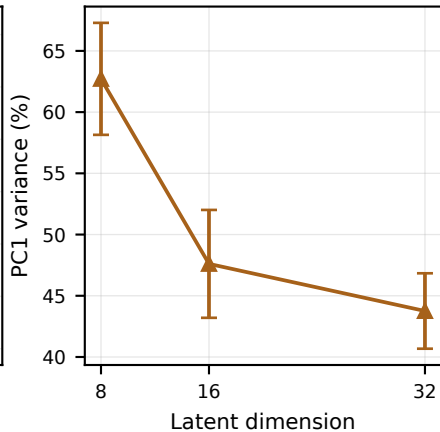
(c) PC1 variance
