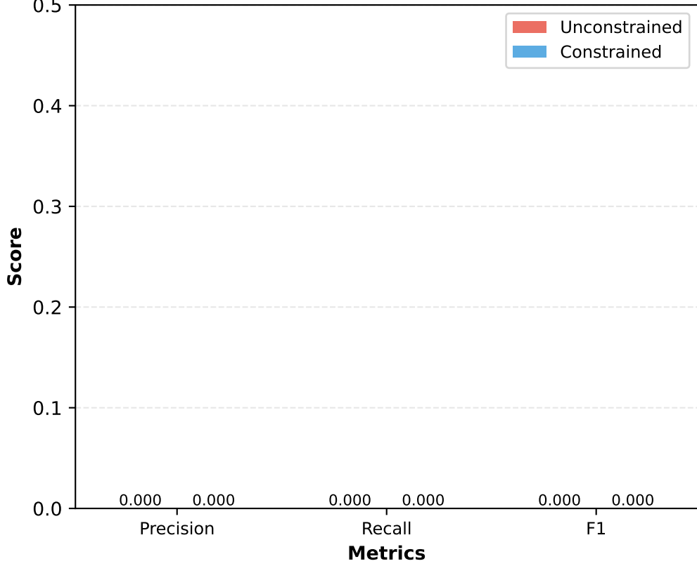
ROUGE-L Details
