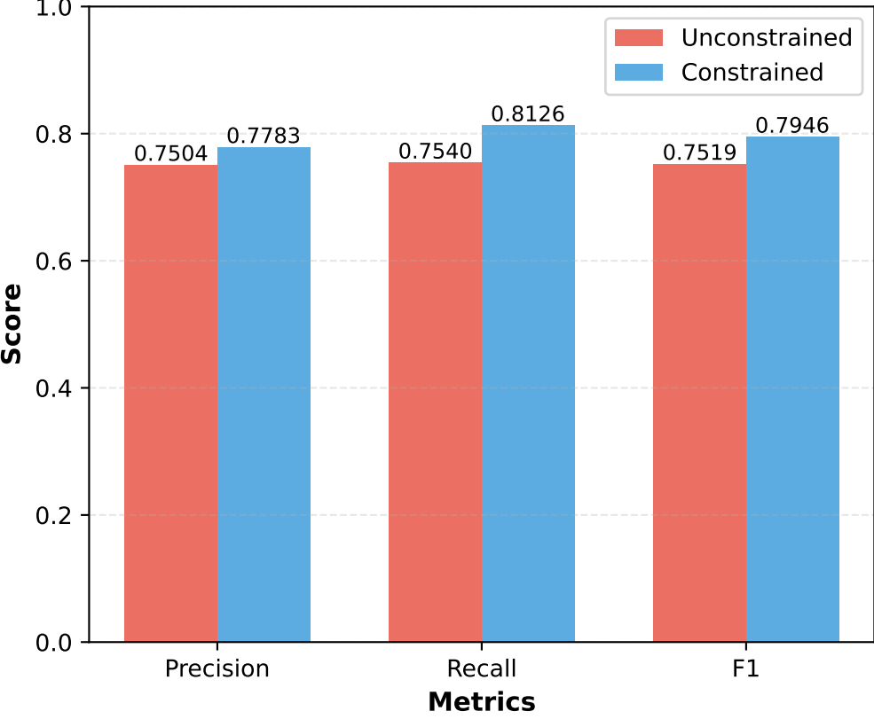
ROUGE-1 Details
