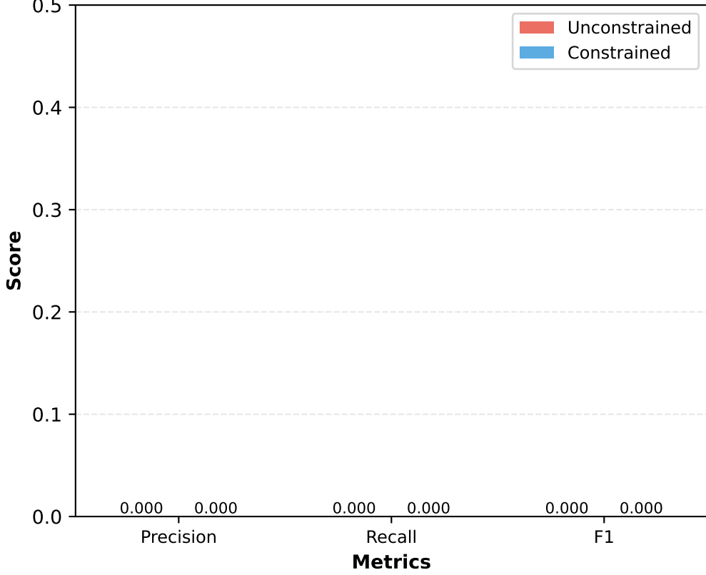
ROUGE-2 Details
