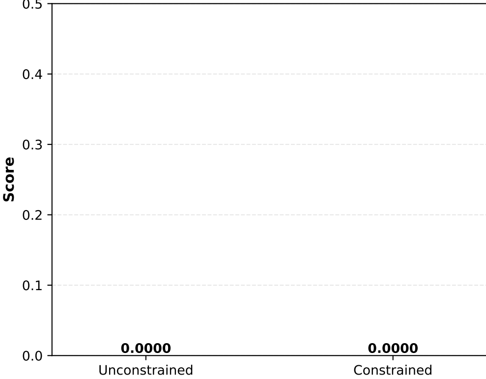
METEOR
