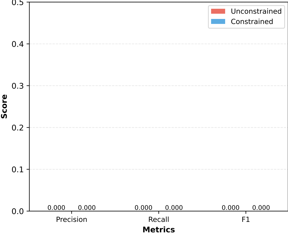
ROUGE-1 Details
