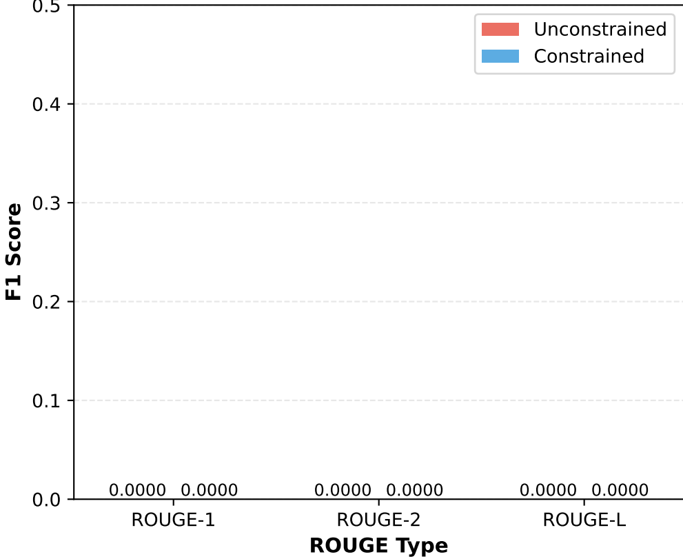
ROUGE-L Details
