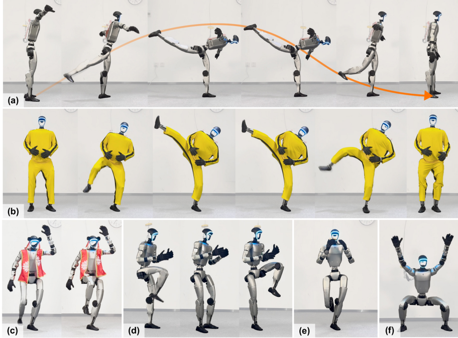
Figure 1: Extreme Balance Tasks. HuB enables humanoids to perform extreme quasi-static balance tasks with high stability. (a) Swallow Balance: holding a challenging T-shaped pose with the torso extended horizontally; (b) Bruce Lee’s Kick: executing a high kick with full leg extension while balancing on one foot; (c) Ne Zha Pose: a martial arts-inspired one-legged stance with a raised arm; (d) High Knees; (e) Single-Leg Stand; (f) Deep Squat. Videos are available at: hub-robot.github.io
