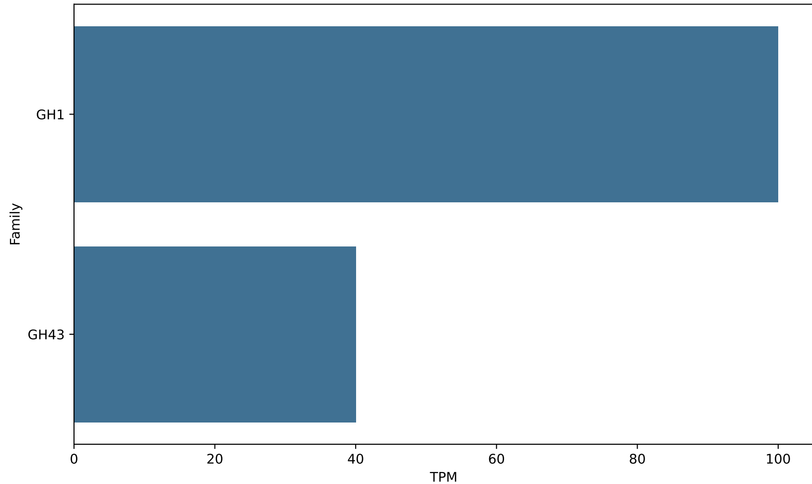
CAZyme abundance
