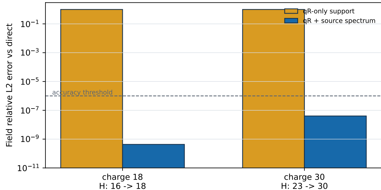
High-NA Debye-Wolf support control
