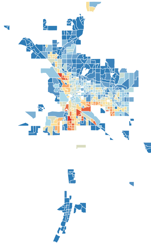
b SSP5-8.5, 2060s
