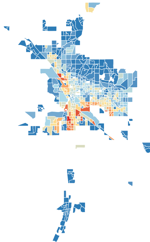
b SSP5-8.5, 2060s
