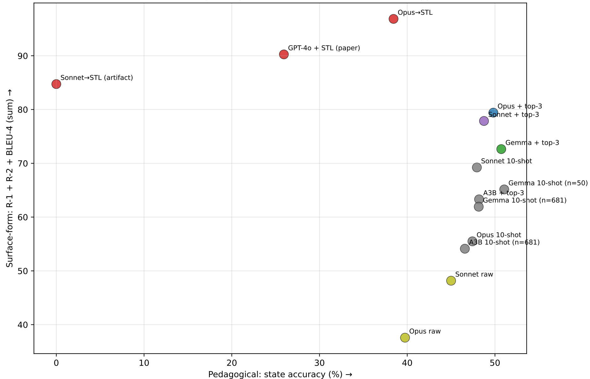
Surface-form metrics vs pedagogical state accuracy (SocratTeachLLM-using configs in red; tracks anti-correlation in upper-left)
