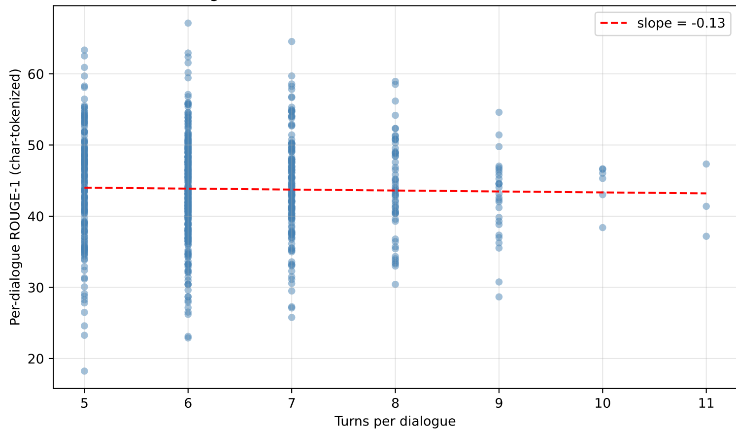
Per-dialogue ROUGE-1 vs turn count — GPT-4o baseline (n=681)
