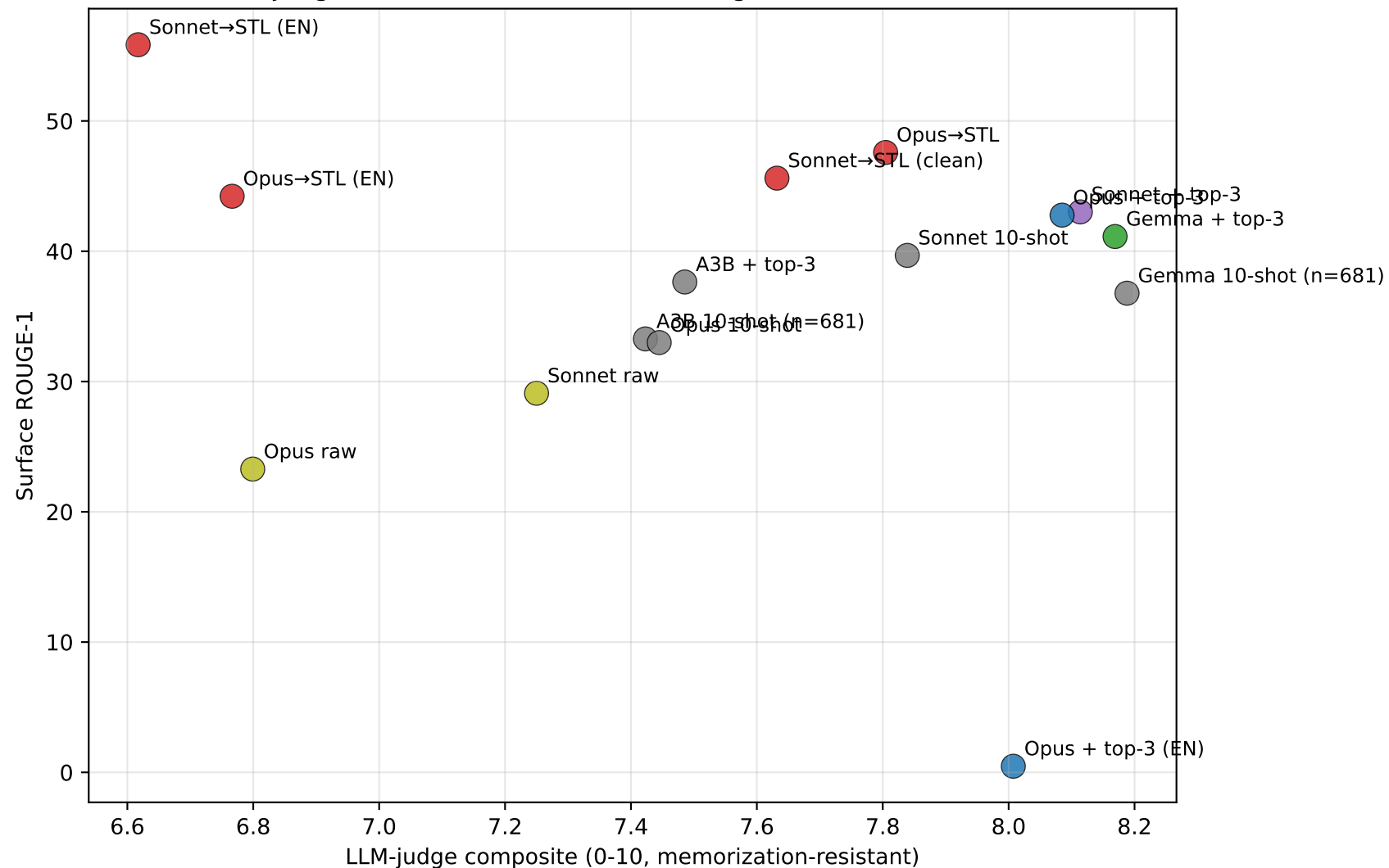
LLM-judge vs surface ROUGE-1 — orthogonal axes of evaluation
