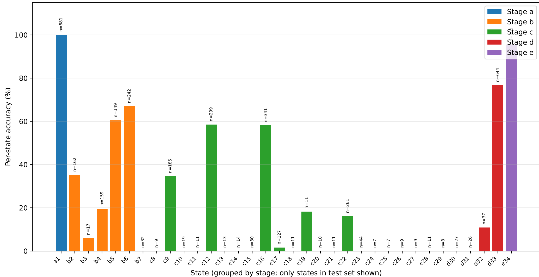
34-state BERT classifier per-state accuracy on test split (overall: 61.64%, n=4,304 turns)
