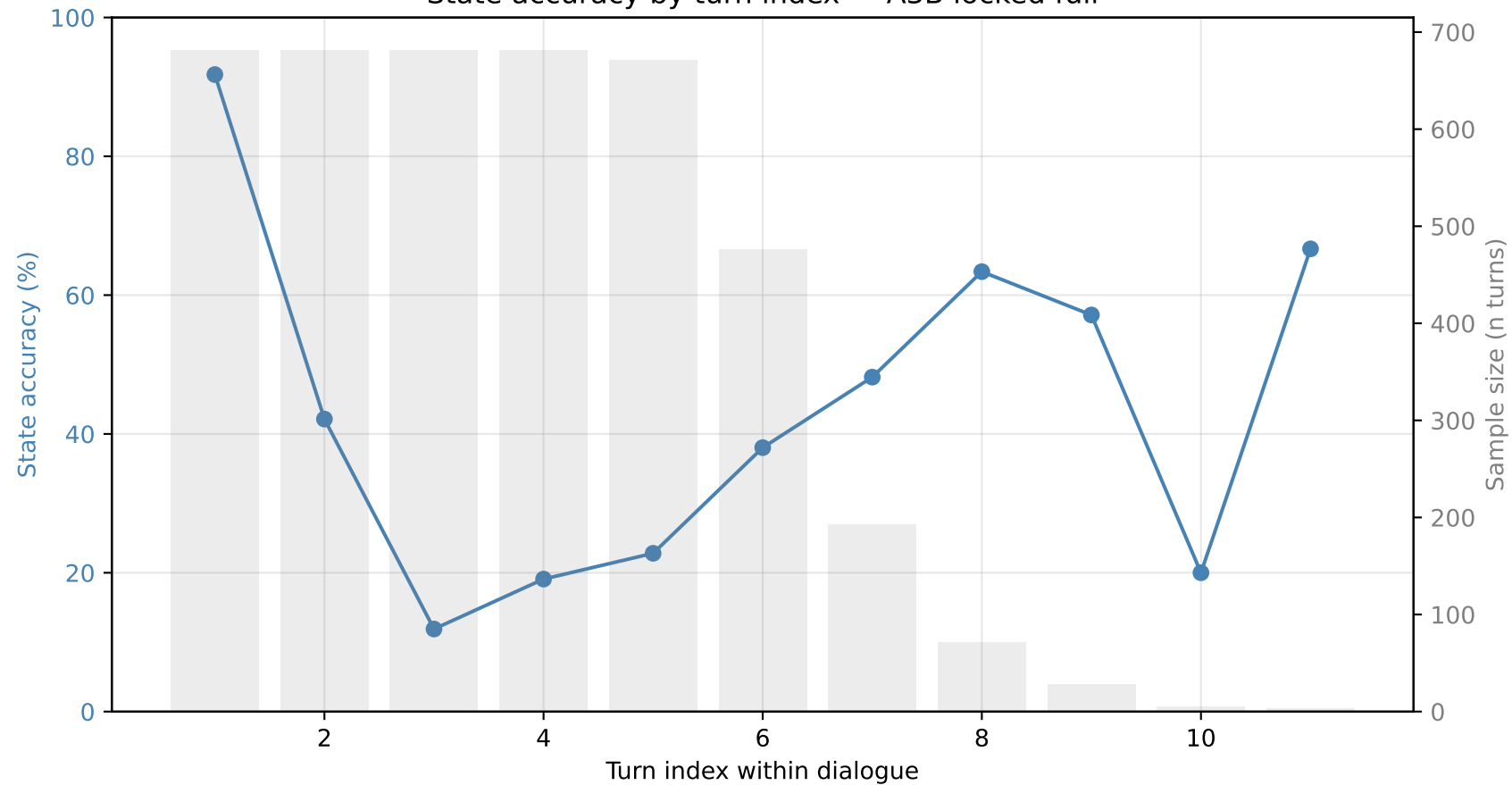
State accuracy by turn index — A3B locked full
