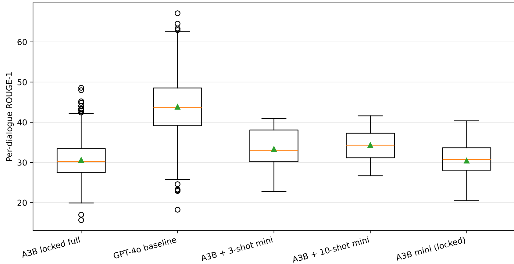
Per-dialogue ROUGE-1 distribution across systems
